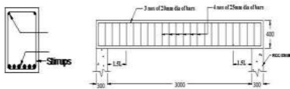
Beam- Reinforcement Details
